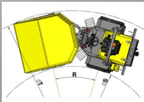
STATIC DIMENSIONS in mm
